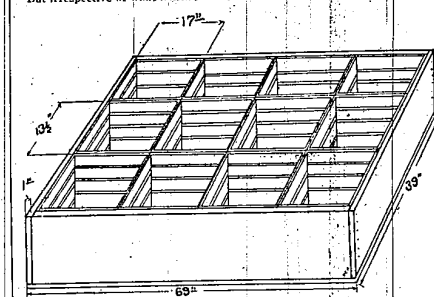
Trough for Handling 12-Bushel Crates of Potatoes; Lined With Canvas to Make It Water-Tight.
