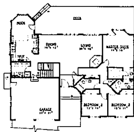
1st/2nd FLR PLAN OVERALL DIMENSIONS: 60'-0" X 54'-0" LIVING: 2005 square feet GARAGE: 545 square feet
