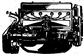
Chevrolet's new six-cylinder, fully enclosed valve-in-head engine meets the 1929 A. S. D. and is developed 60 H. P. at low engine speed.
