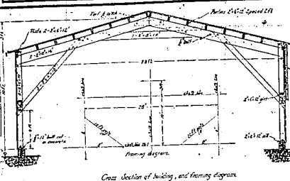
Cross section of building, and framing diagram.
