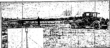
Above: The 122-foot pole on the way from Lawrenceville, N. J., to the radio telephone station at Forked River, showing the highway trailer supporting the rear section of the pole. This trailer, was equipped to be steered around corners independently of the steering of the truck. Left: The pole in place as a radio telephone antenna.
