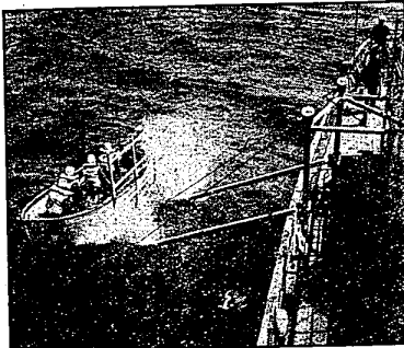
CRADLE OF THE DEEP —A Coast Guard lifeboat splashes into the sea in a test of a revolutionary new cradle device, by means of which a boat can be launched in five seconds. Launching time with conventional davits ranges from 30 seconds to three minutes. Based on an air hoist principle, the cradle swings outward and down from the ship's side, sinking beneath the surface as the boat floats clear.
