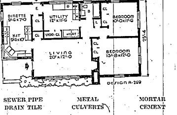
A SMALL HOUSE PLANNING BUREAU DESIGN NO. A-269
