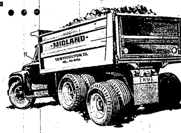
Factory-built tandem-axle T-800, 42,000 lbs. GVW, 65,000 lbs. GCW. Choice of two V-8's with up to 212 h.p.
