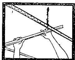
SUSPEND gridwork at desired height...
