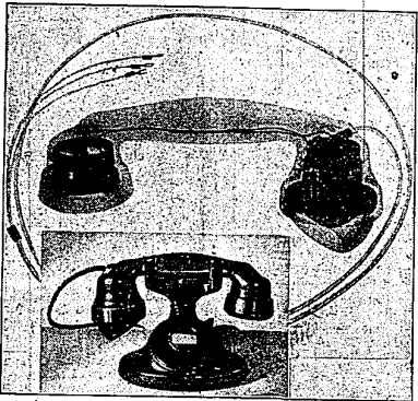
This X-ray photograph of a telephone hand set, made at the Bell Telephone Laboratories, reveals clearly the positions of the transmitter and receiver units and the conductors in their solid molded frame. The smaller picture shows the hand set as it appears to human eyes. Scientists at the Bell Laboratories make frequent use of X-ray photography for studying the structure of metals and other solids.
