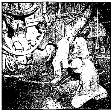
UNDERWATER REPAIR JOB —The Grand Coulee Dam, on the Columbia River, undergoes a face-lifting with the aid of a special underwater chamber that permits workmen to labor 70 feet under water. The men are making repairs to the spillway bucket of the 22-million-ton dam. The underwater chamber is lowered over the bucket and water is pumped out so that workers can go below.
