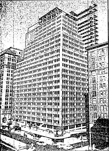
THIS AGE OF SPEED —Latest addition to New York's Park Avenue skyscrapers donned its prefab skin in a record-breaking six-and-one-half working days. Three specially trained crews clad the 26-story skeleton of steel and concrete with 1800 prefabricated aluminum panels. Each panel contains two six-foot windows which rotate for safe interior cleaning. Ordinary brick-and-mortar construction would have necessitated eight weeks for completion.
