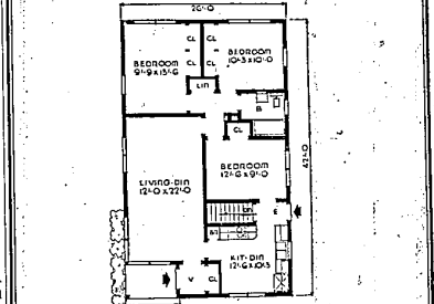
A SMALL HOUSE PLANNING BUREAU DESIGN No. C-352
