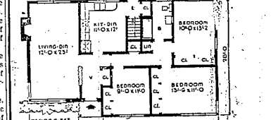
A SMALL HOUSE PLANNING BUREAU DESIGN NO. C-342
