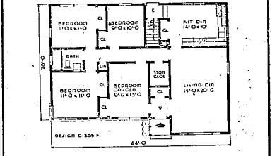
A SMALL HOUSE PLANNING BUREAU DESIGN NO. C-385-F
