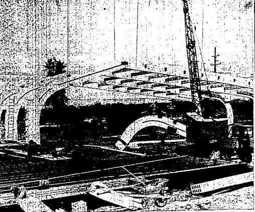
A MODERN addition to the commercial district at Ten Mile and Orchard Lake Road is now going up. Forming the framework for the new Bel-Aire bowling alley being constructed on Orchard Lake just south of Leelanau are these large pre-cast trusses. They were being set in place last week. The building is scheduled for completion in time for the opening of the bowling season next fall.
