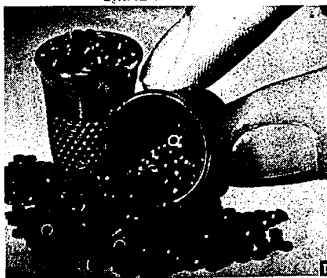
These tiny doughnut-like cores, the electro-magnetic building blocks for many modern computer memories, are made by IBM in almost microscopic sizes. A typical computer memory might contain more than a million such cores. Each is separately tested during production.
