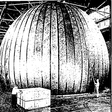
BIG THING IN A SMALL PACKAGE —Believe it or not, this 36-foot-high radome with a 167-foot circumference fits in the wooden crate at left. Designed to safeguard radar installations from the elements, the rubberized fabric hemisphere was inflated in an Akron, O. factory before being shipped to the Air Force. It requires no rigid supports and only a twentieth of a pound of air pressure to hold its shape.
